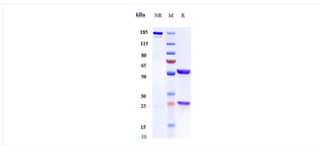
Anti-IL-4 Reference Antibody (pascolizumab) on SDS-PAGE under reducing (R) condition. The purity of the protein is greater than 90%.
