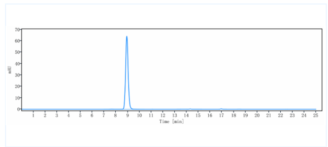
The purity of Anti-IL-4 Reference Antibody (pascolizumab) is more than 95%, determined by SEC-HPLC.
